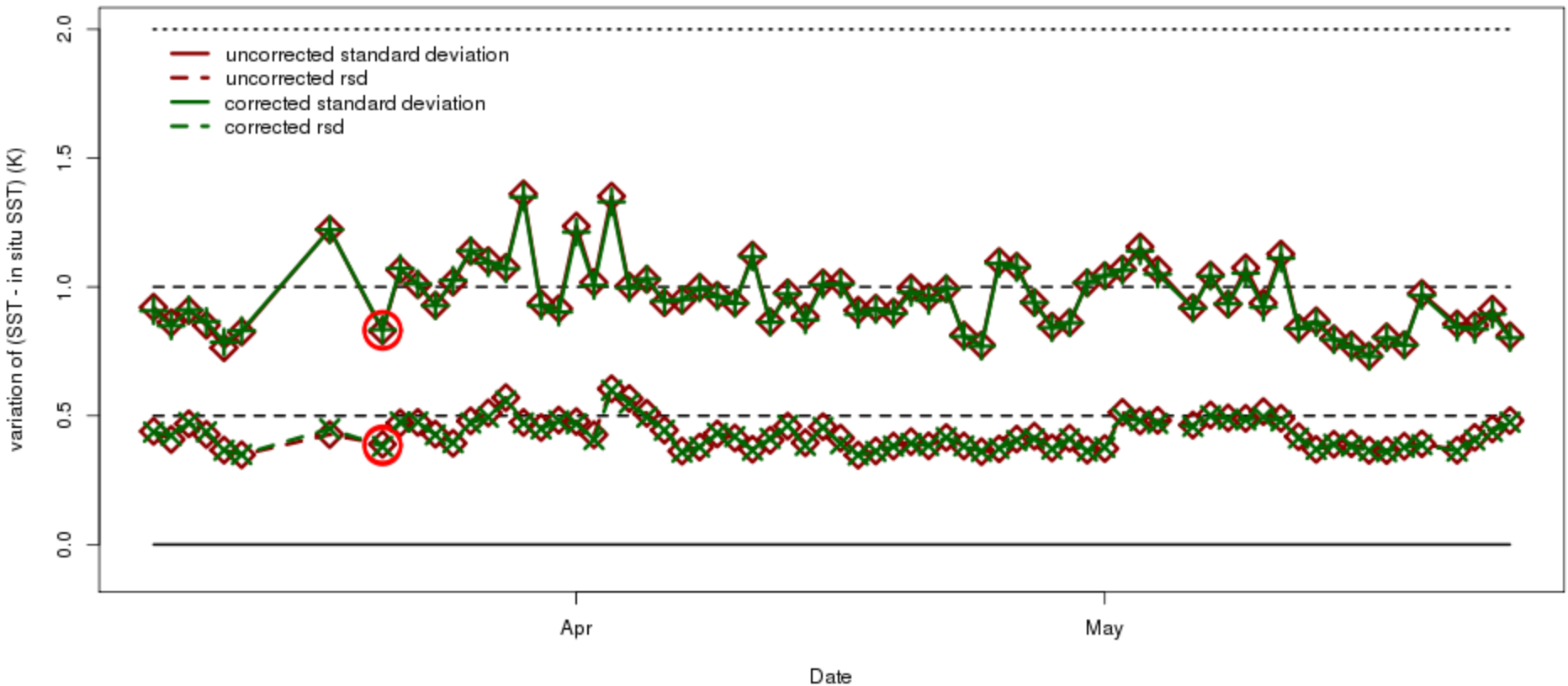
GHRSSST L2P LRG2.12 HW8 SST Single (Day and Night) Algorithm, daily (day time) Deviations Himawari-8 , last 78 days, 2016-03-08 to 2016-05-24
