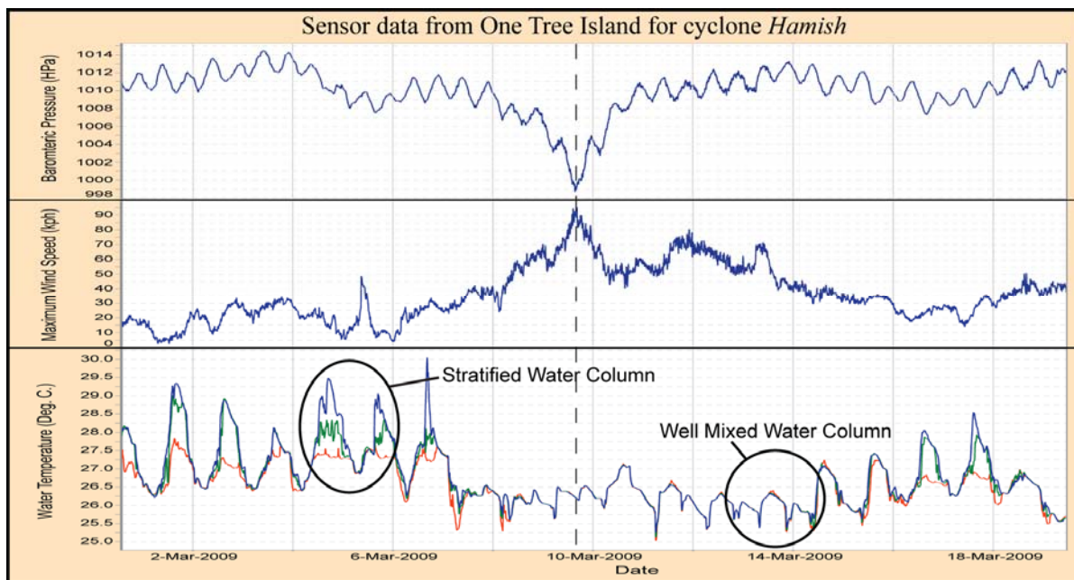
Figure One. Real time sensor network data showing the impact of cyclone Hamish at One Tree Island. Top graph is atmospheric pressure, middle graph is wind speed, bottom graph is a temperature profile showing how the stratified lagoon becomes well mixed.
